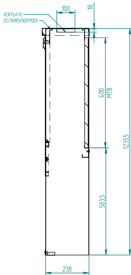
SECTION C-C
